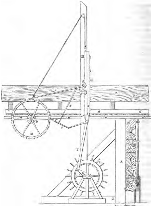
AMERICAN SAW MILL.
